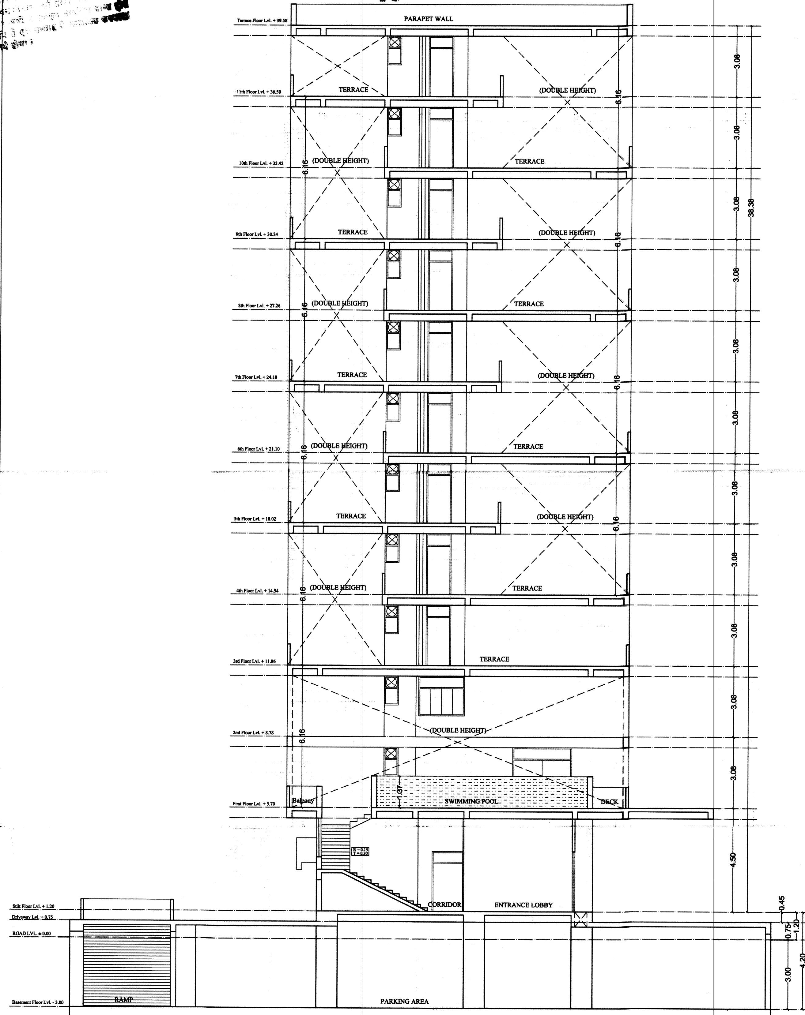
SECTION AT S1-S1
