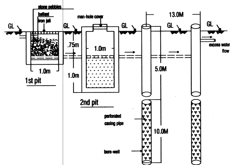
SECTION THROUGH R.W. HARVESTING PITS
